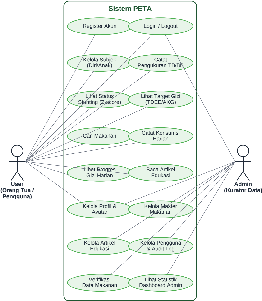
Gambar 1. Use Case Diagram Sistem PETA (User & Admin).
